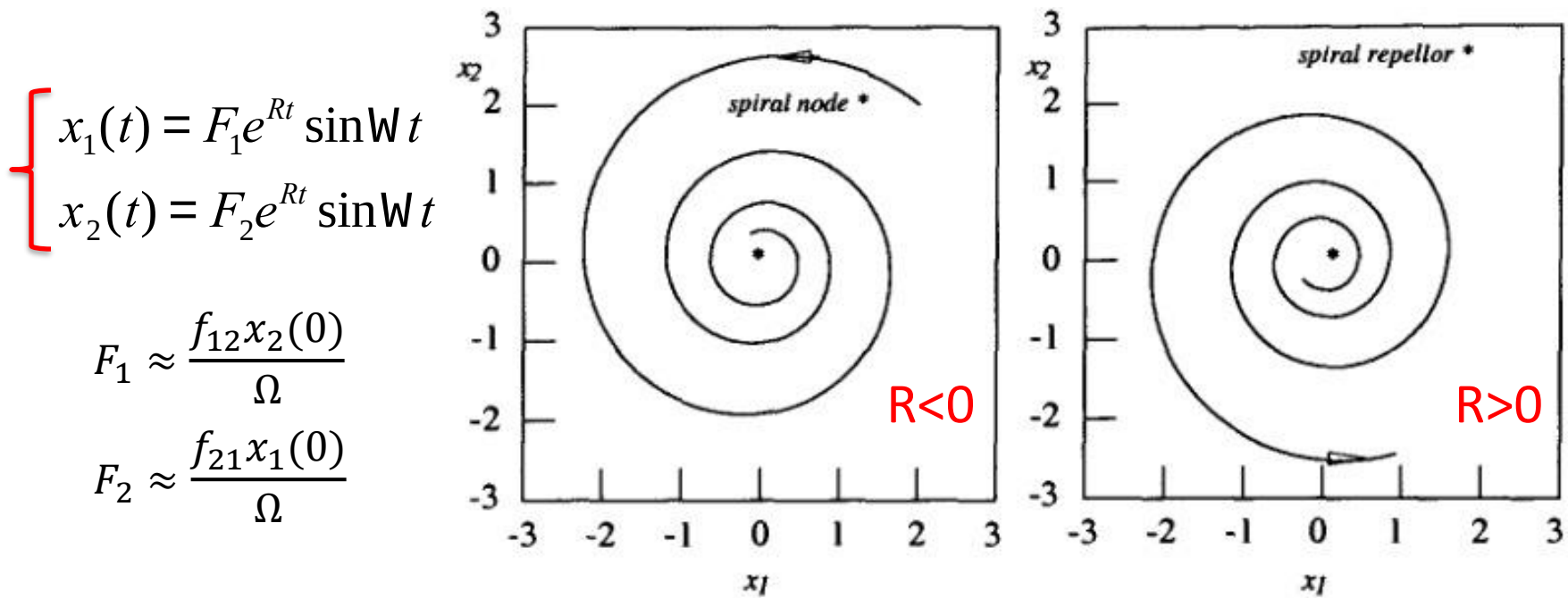
Fig. 3.10. A spiral node (left) and a spiral repeller (right) occur when the characteristic values of a fixed point are complex numbers.
